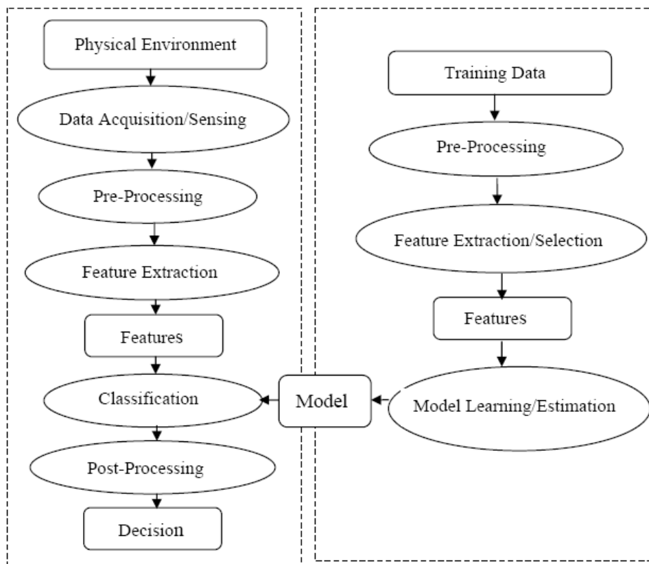
Fig. 1 Conventional Framework of Pattern Recognition System [11]
